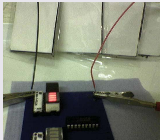
Figure 2. Lithographically printed battery powering 'conventional' circuit
