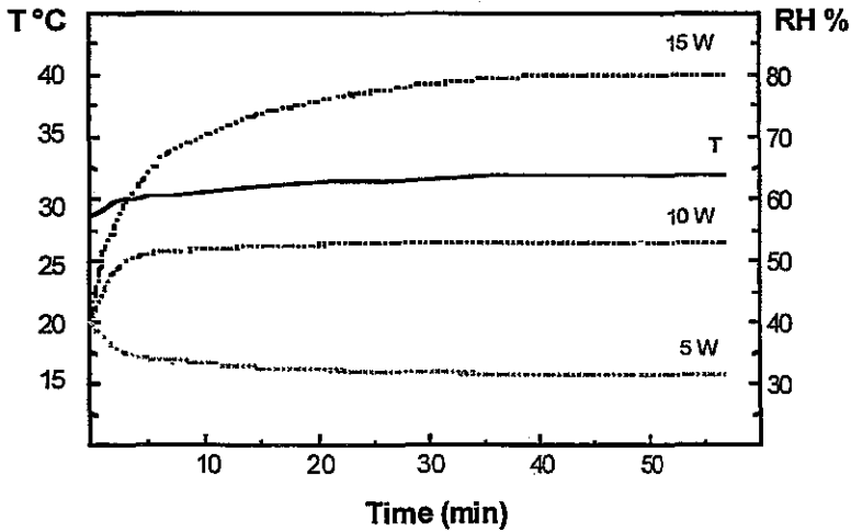
Figure 3. Fuzzy-controlled adjustment of relative humidity (dotted lines) inside a trekking shoe at different levels of workload. The measured temperatures (filled line) are identical at every level of workload (5W/10W/15W).
