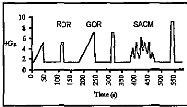
Figure 1. Acceleration profile.
