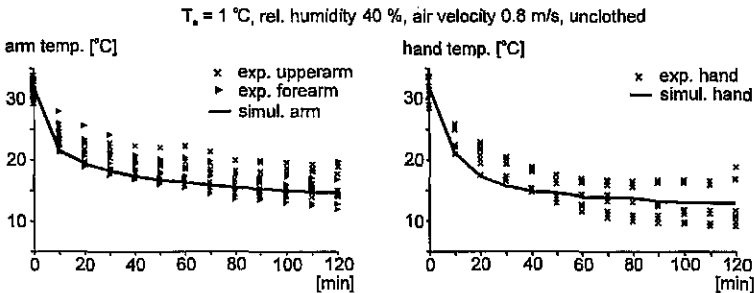
Fig. 4: Comparison of experimental and computational results (THERMOSIM)
