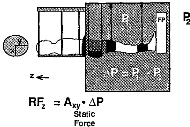
Figure 1: Reaction force ( RF_z ) to generate body weight in supine posture equals the product of the cross-sectional area of the flexible waist seal ( A_{xy} ) and the suction pressure ( \Delta P ) as measured by a force plate (FP) within the LBNP chamber. With exercise, inertial RF_z s are added to the static force.
