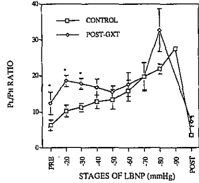
Figure 2. P_1/P_H ratio as a function of LBNP stage for the control and post-GXT condition. Values expressed are means \pm 1 SE. * indicates a significant difference from control ( P < 0.05 ).
