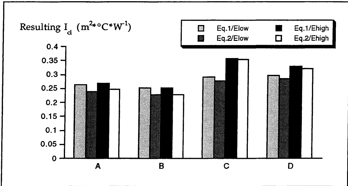
FIGURE 1. Resulting basic insulation of four clothing ensembles calculated with alternative equations.
