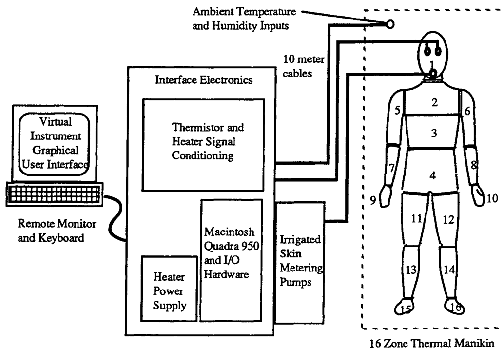
Figure 1 - Heat Pipe Thermal Manikin System
