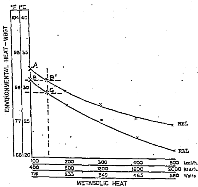
Figure 1. Recommended Heat-Stress Alert Limits (RAL) and Exposure Limits (REL), (NIOSH, 1986)
