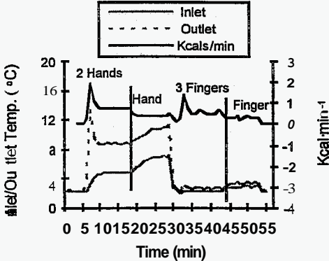
Figure 2. Suit Temperature Inlet/Outlet and Heat Absorption Profile (kcal·min -1 ) by Gloves and Fingers Calorimeter (Female, age 32).
