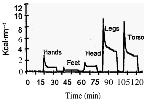
Figure 4. Maximal Heat Flux from Different Parts of the Body Under Cooling Suit at 8°C (Female, age 40).
