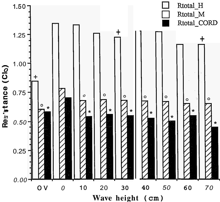
Figure 1. Effect of wave height and vertical immersion posture on the total thermal resistance ( R_{total} ) of the suit system worn by the human subjects and the thermal manikin during immersion in 16°C water. *, °, †: significantly different ( p < 0.05 ) from the 0 cm wave height condition.
