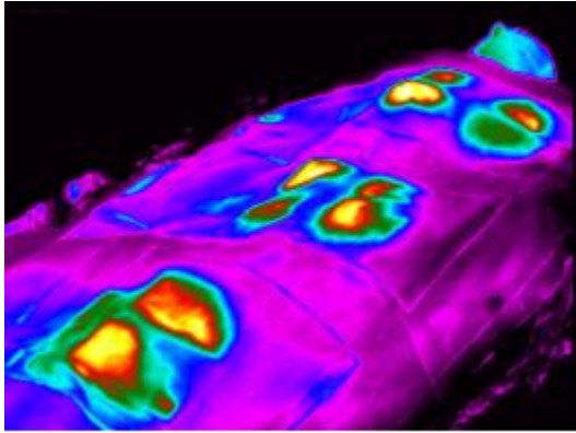
Figure 3. IR Image of the Chemical Blanket and Photo of the Outer Radiation Shield
