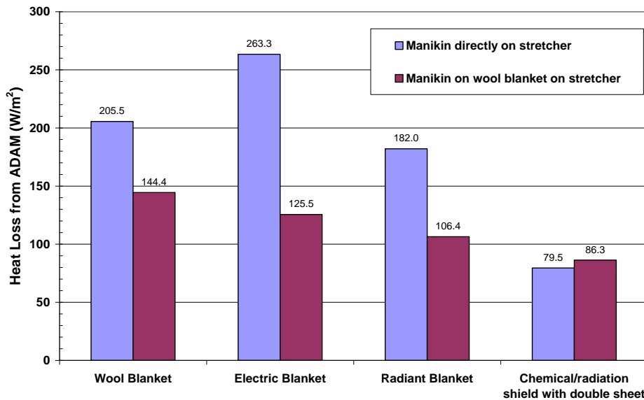
Figure 6. Impact on Heat Loss of Placing a Wool Blanket under the Manikin
