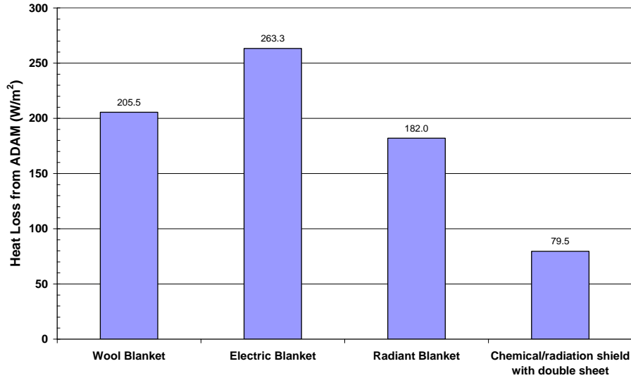
Figure 4. Steady-State Heat Loss with 40°C Skin Temperature
