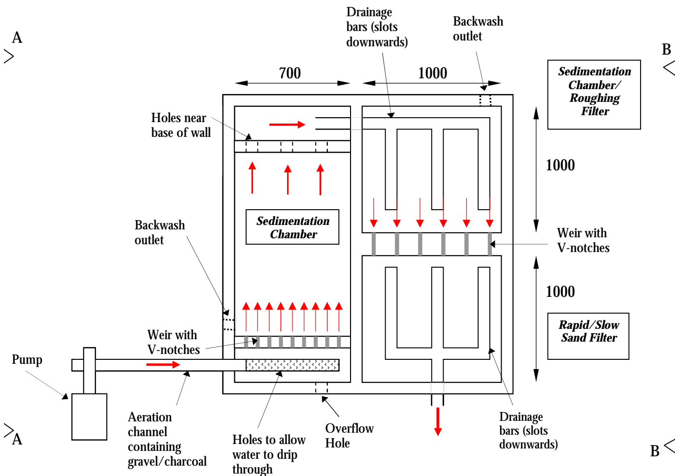
Figure 5 Plan View of Proposed Filter Design
