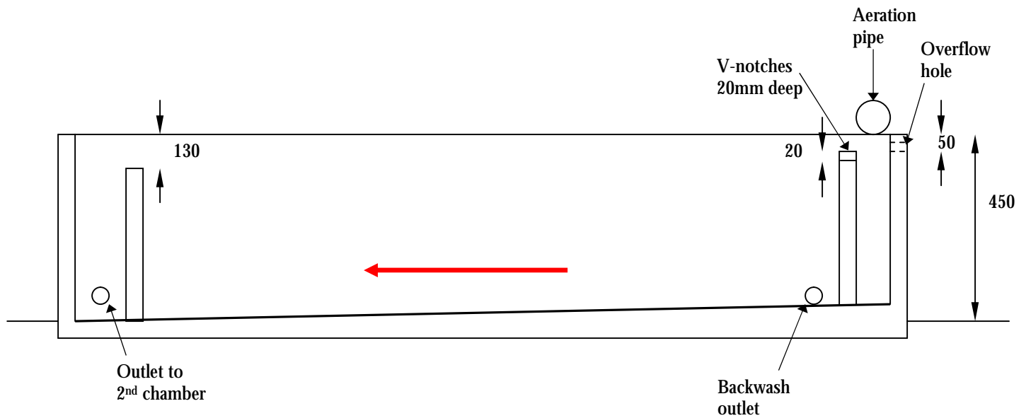
Figure 6 Elevation View of Sedimentation Chamber
