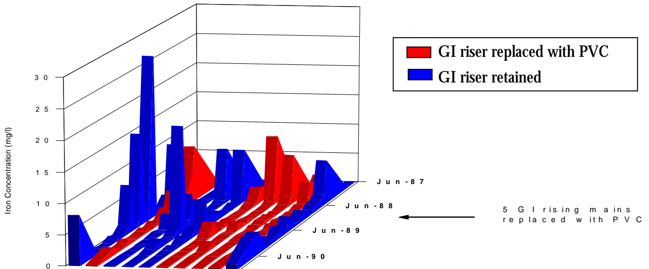
Figure 3 Total Iron content from India Mark II pumps – GI and PVC pipes
