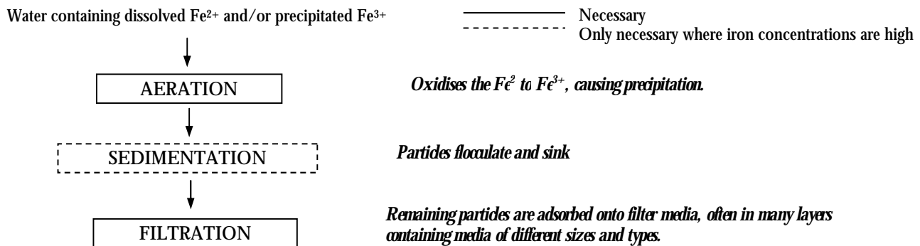
Figure 1 The Iron Removal Process
