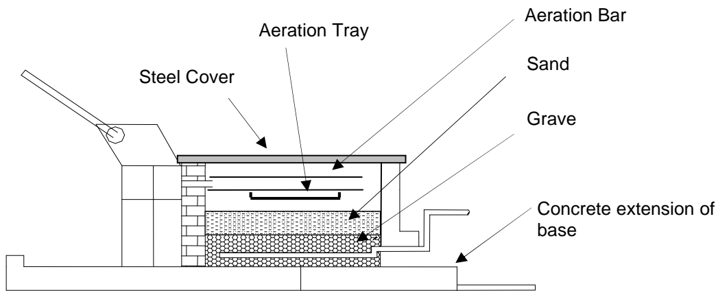
Figure 4 Elevation of the Silsoe Filter as at Bugambe
