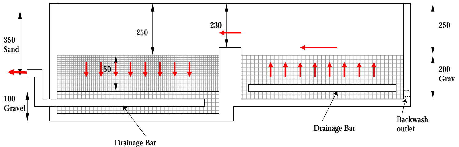
Figure 7 Elevation View of Filter Chambers
